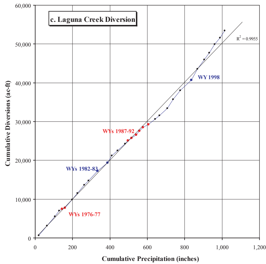
North Coast Precipitation-Diversion Double Mass Curves, WYs 1972-2004
