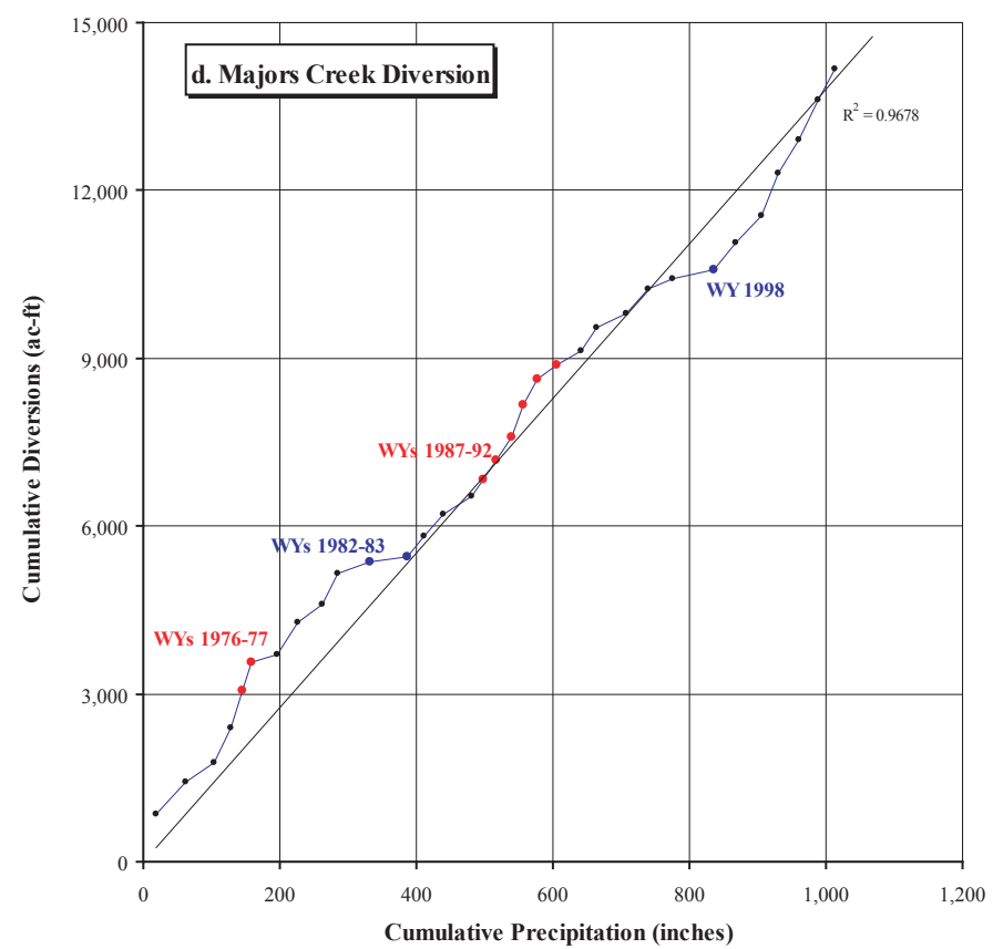
North Coast Precipitation-Diversion Double Mass Curves, WYs 1972-2004
